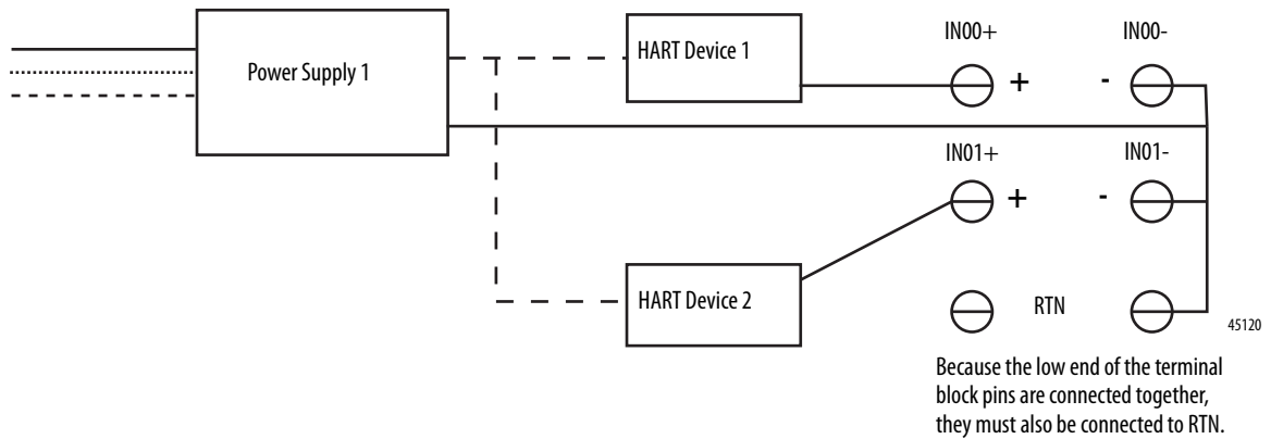
Figure 17 - Single Power Supply with Multiple HART Devices
