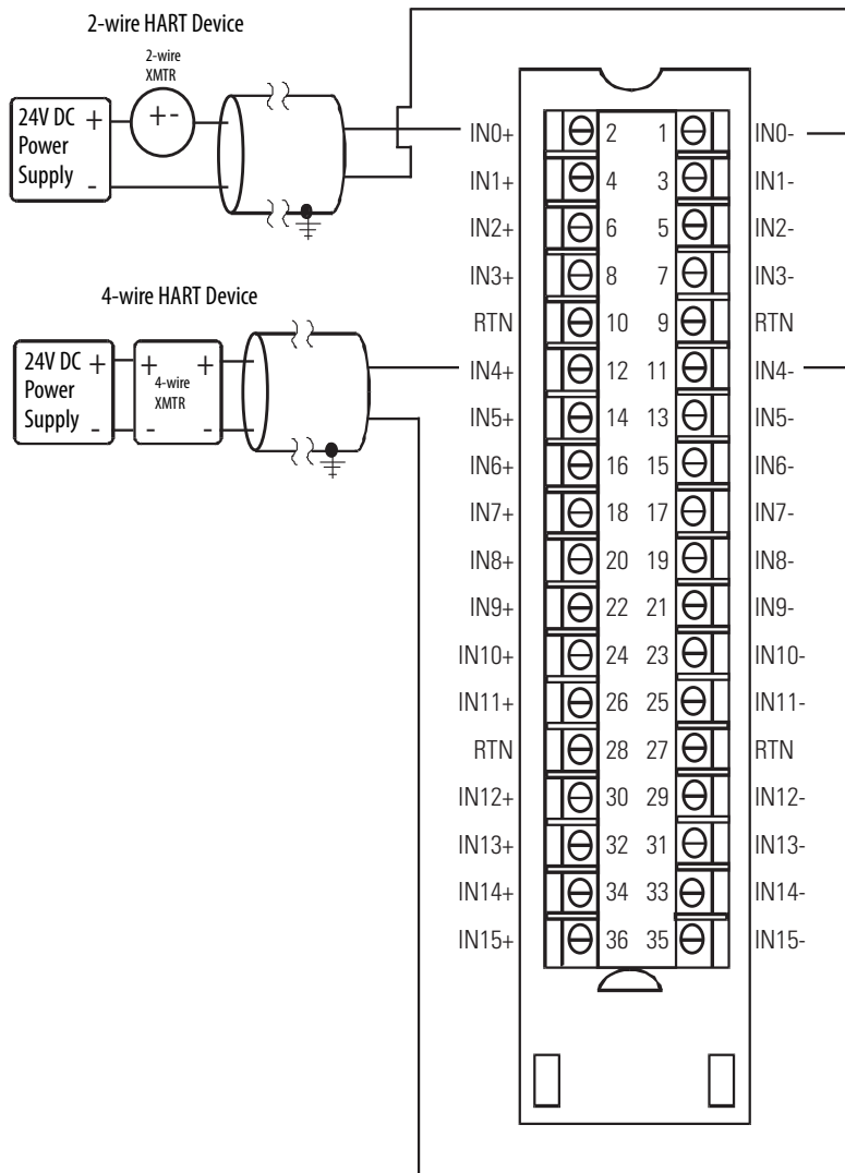
Figure 16 - Current Inputs
