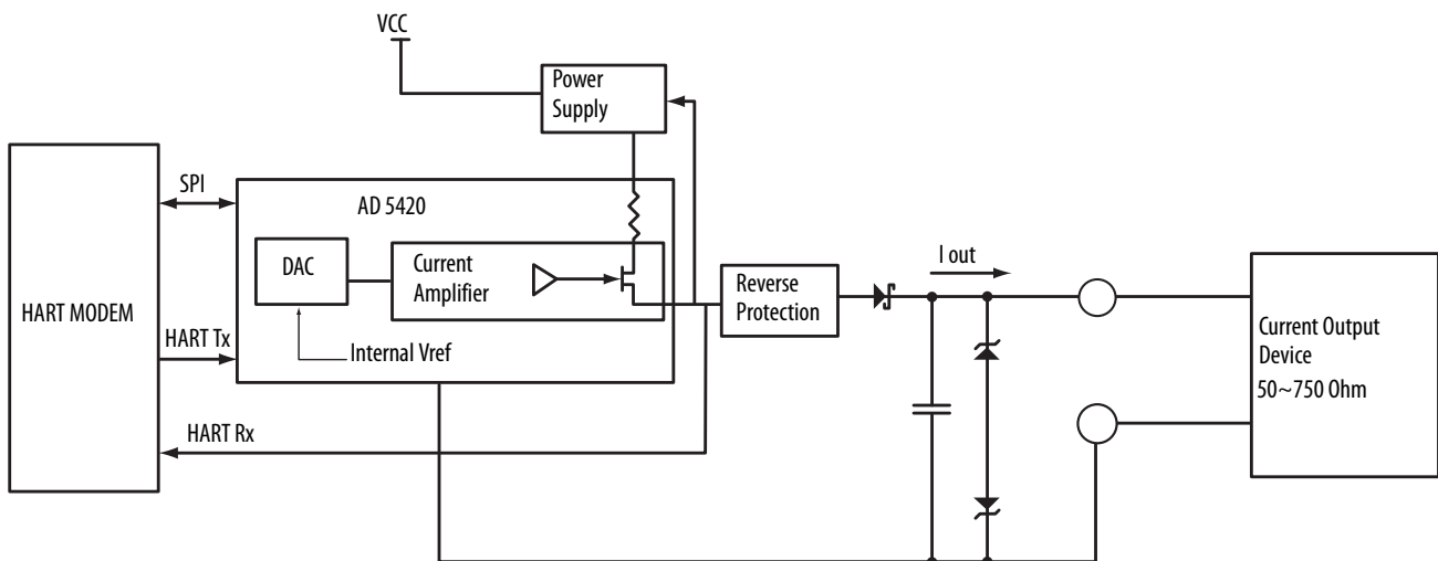
Figure 30 - 1756-OF8IH Output Circuit Diagram
