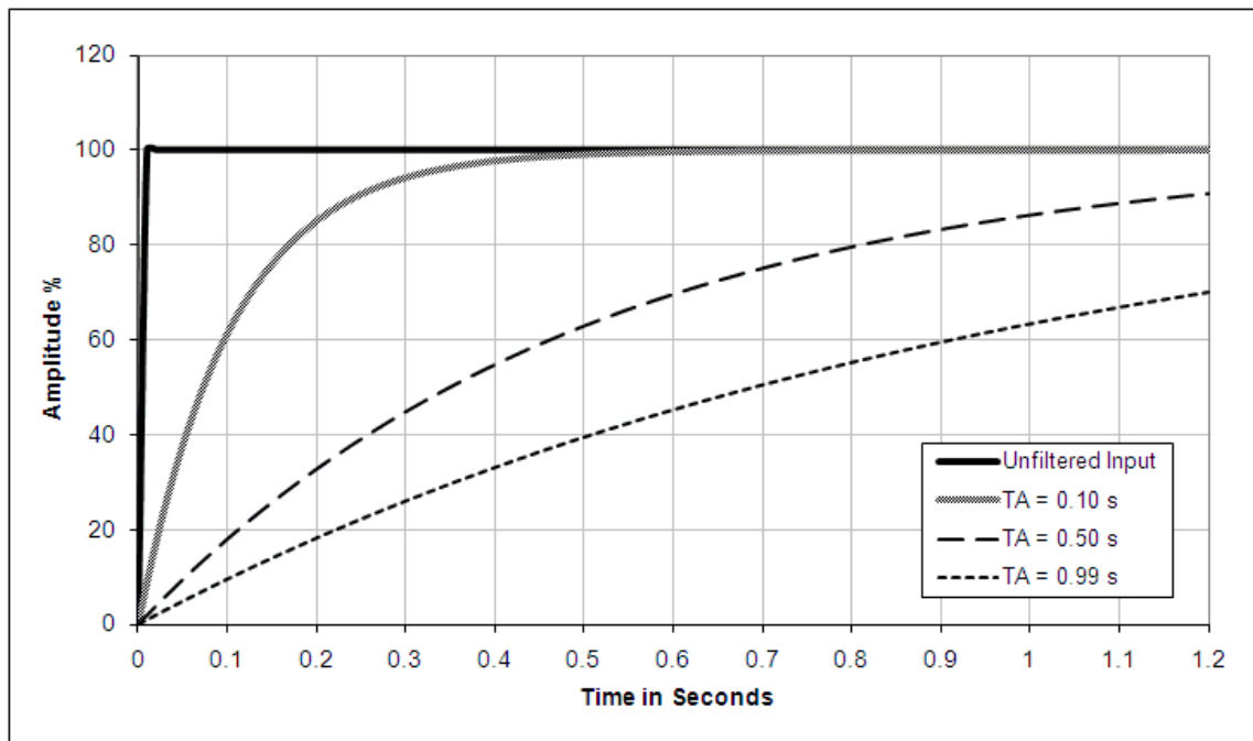
Figure 22 - Filter Response
