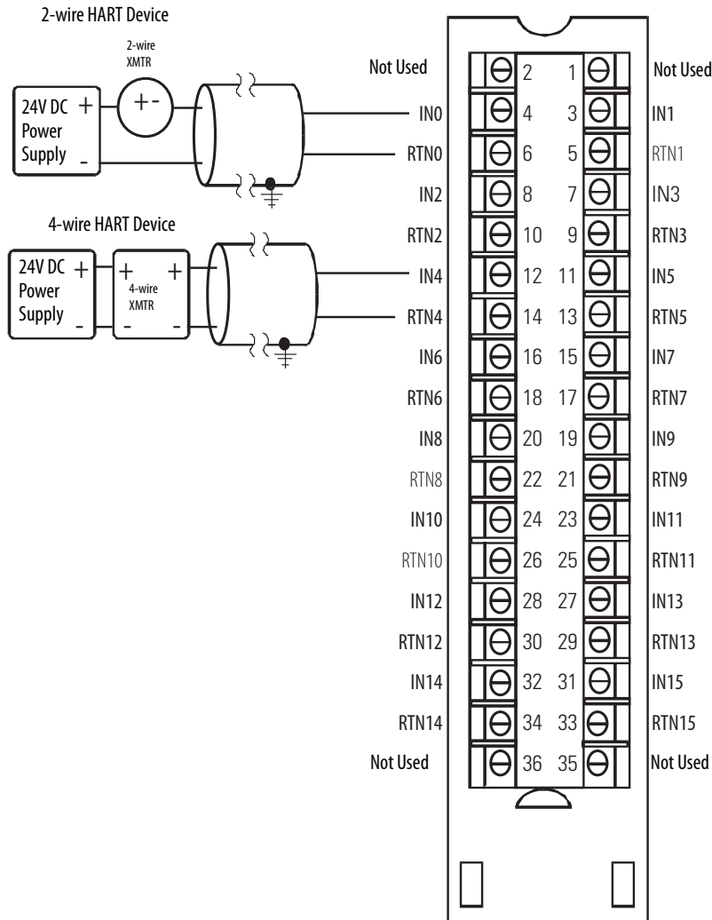
Figure 23 - Current Inputs
