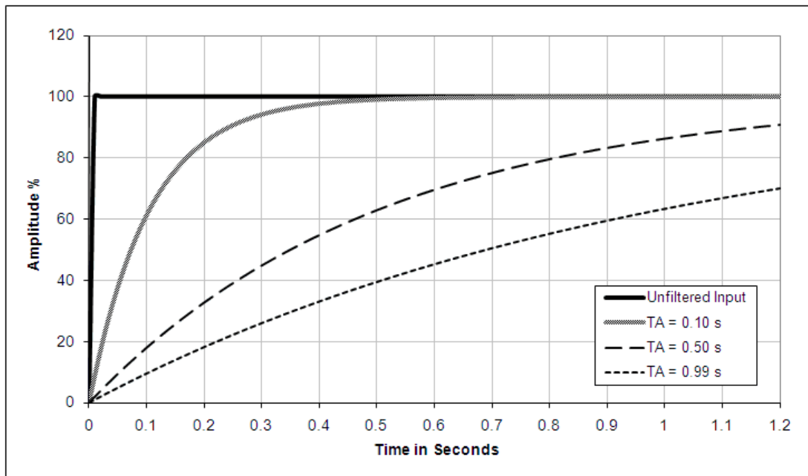
Figure 2 - Filter Response
