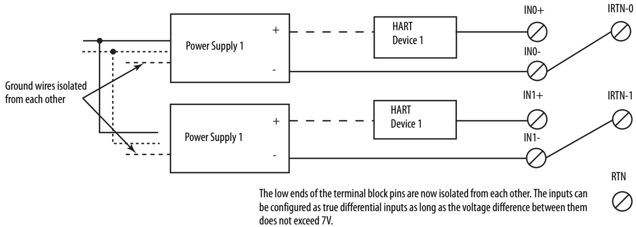
Figure 7 - Power Supplies with Isolated Grounds
