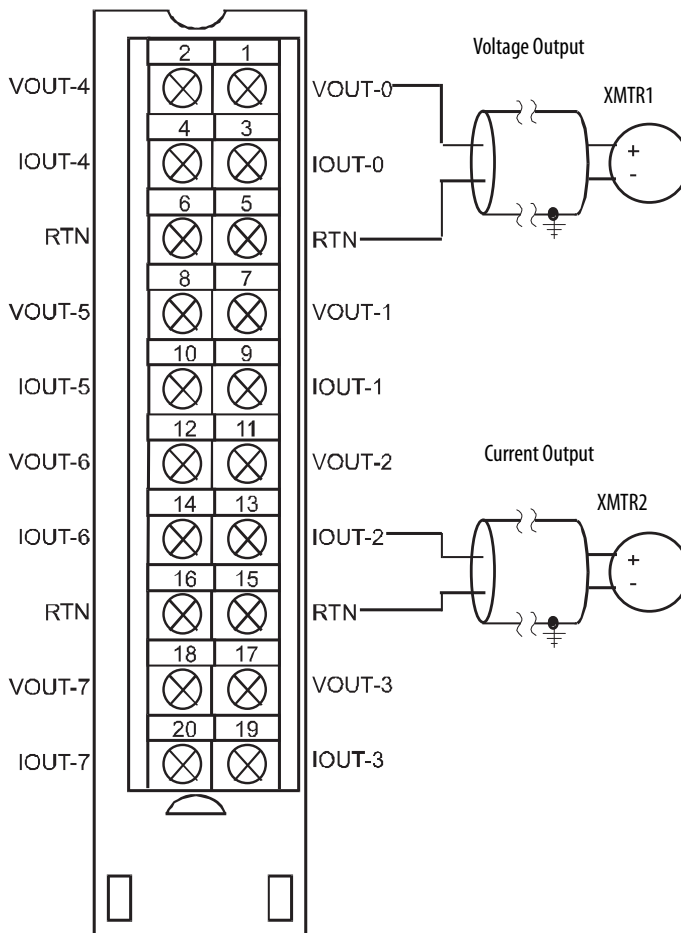
Figure 26 - Wiring Diagram for the 1756-0F8H Module
